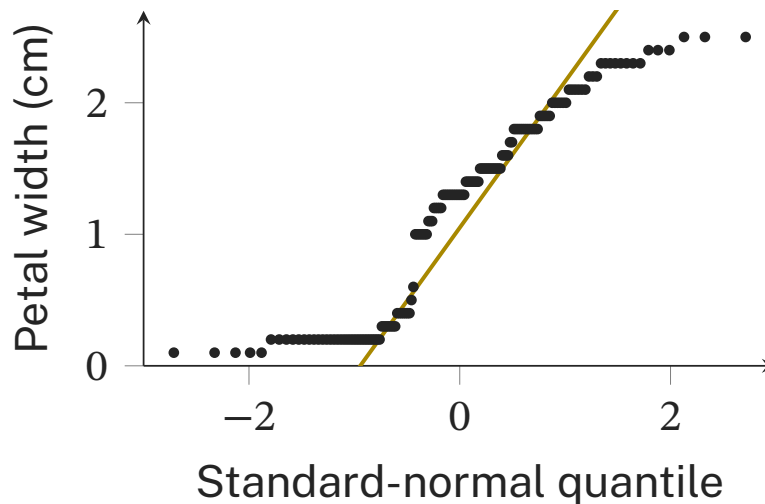
Figure 16. Iris petal-width normal Q-Q plot using the stated plotting positions and a quartile reference line with slope 1.11195 cm and intercept 1.05 cm.
